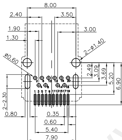
RECOMMENDED PCB LAYOUT TOLERANCE: ±0.05 TOP VIEW
